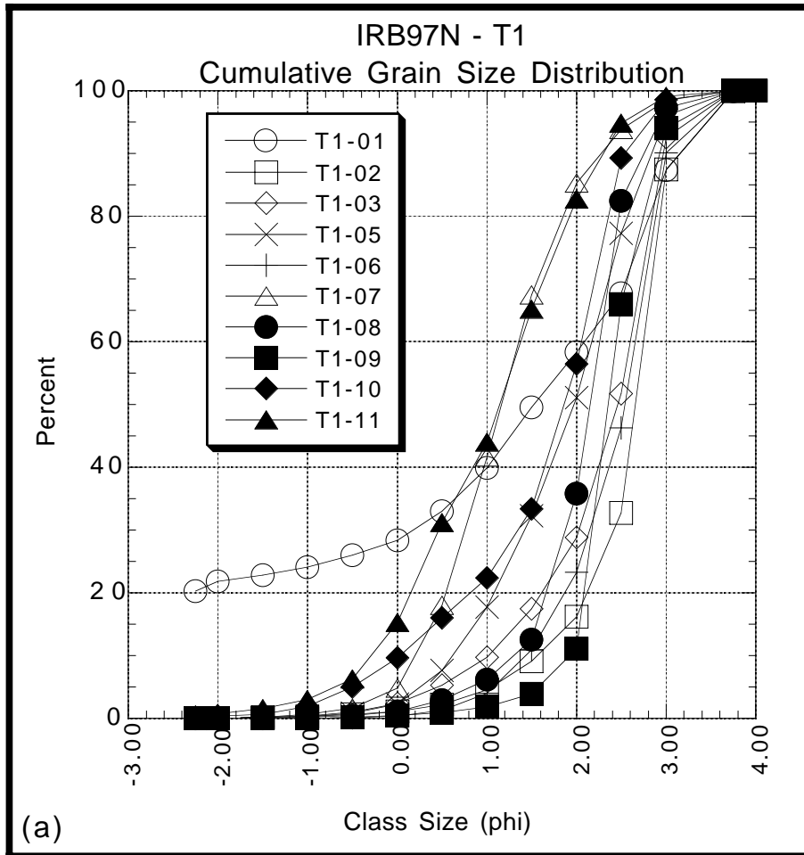
Figure 53. Cumulative frequency grain size distribution, IRB97N. (a) Transect 1 sediment samples. (Continued on next page.)
