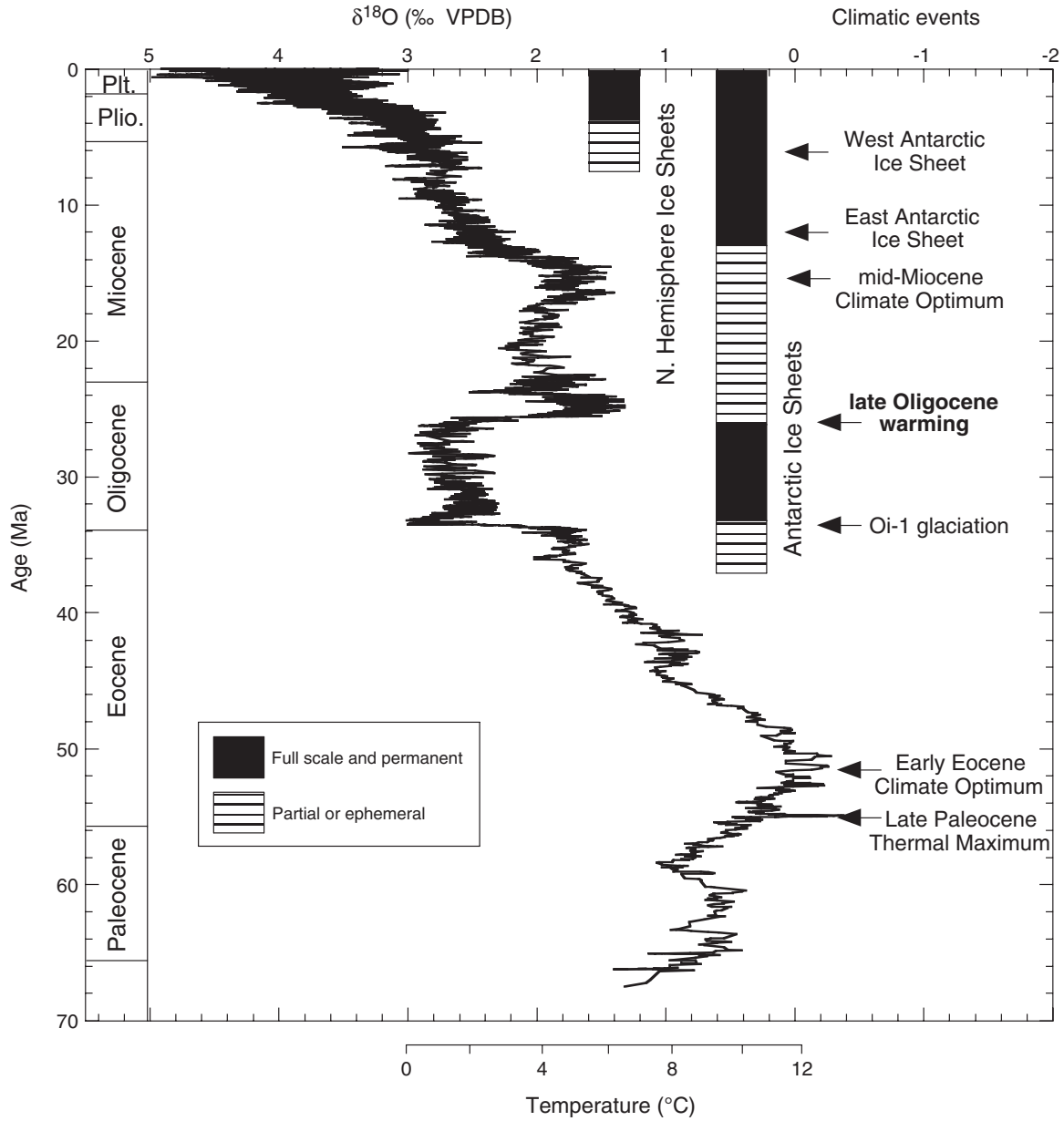
Figure F1. Compilation of benthic oxygen isotope data from Cenozoic deep-sea cores (after Zachos et al., 2001). Note prominent \delta^{18}\text{O} decrease of >1\text{‰} during the late Oligocene at \sim 26 Ma against the long-term Cenozoic \delta^{18}\text{O} increase. VPDB = Vienna Pee Dee belemnite.
