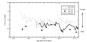
F6. \delta^{13}\text{C} data vs. age, p. 15.
