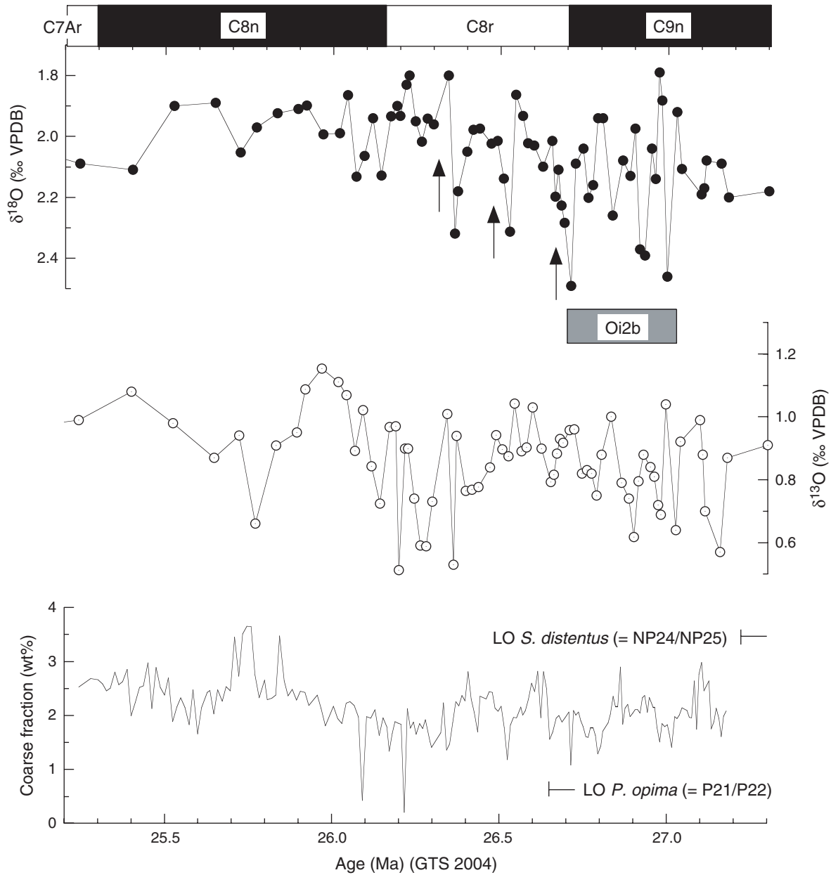
Figure F5. Stable isotope (based on Cibicidoides mundulus ) and percent coarse fraction (weight percentage of the >63- \mu\text{m} fraction) data vs. age in million years before present (Ma) in Core 202-1237B-31H. Also shown are paleomagnetic Chrons 7Ar to 9n (Gradstein et al., 2004) and last occurrence (LO) of the calcareous nannofossil Sphenolithus distentus (Shipboard Scientific Party, 2003) and LO of the planktonic foraminifer Paragloborotalia opima (this study). The initiation of the Chron 8r \delta^{18}\text{O} shift is associated with LO of P. opima . VPDB = Vienna Pee Dee belemnite.
