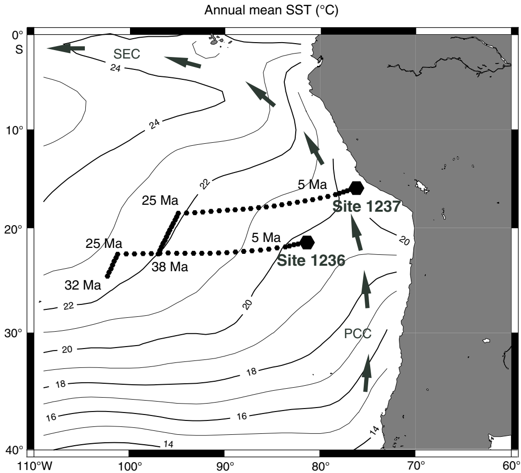
Figure F2. Location map (Shipboard Scientific Party, 2003) showing Sites 1237 and 1236 on Nazca Ridge and their tectonic backtrack paths, plus annual mean sea-surface temperature (SST). Note that Site 1237 was within the subtropical South Pacific gyre during the late Oligocene. Also shown are positions of the Peru-Chile Current (PCC) and the South Equatorial Current (SEC).
