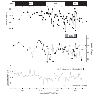
F5. \delta^{18}\text{O} and coarse fraction data vs. age, p. 14.
