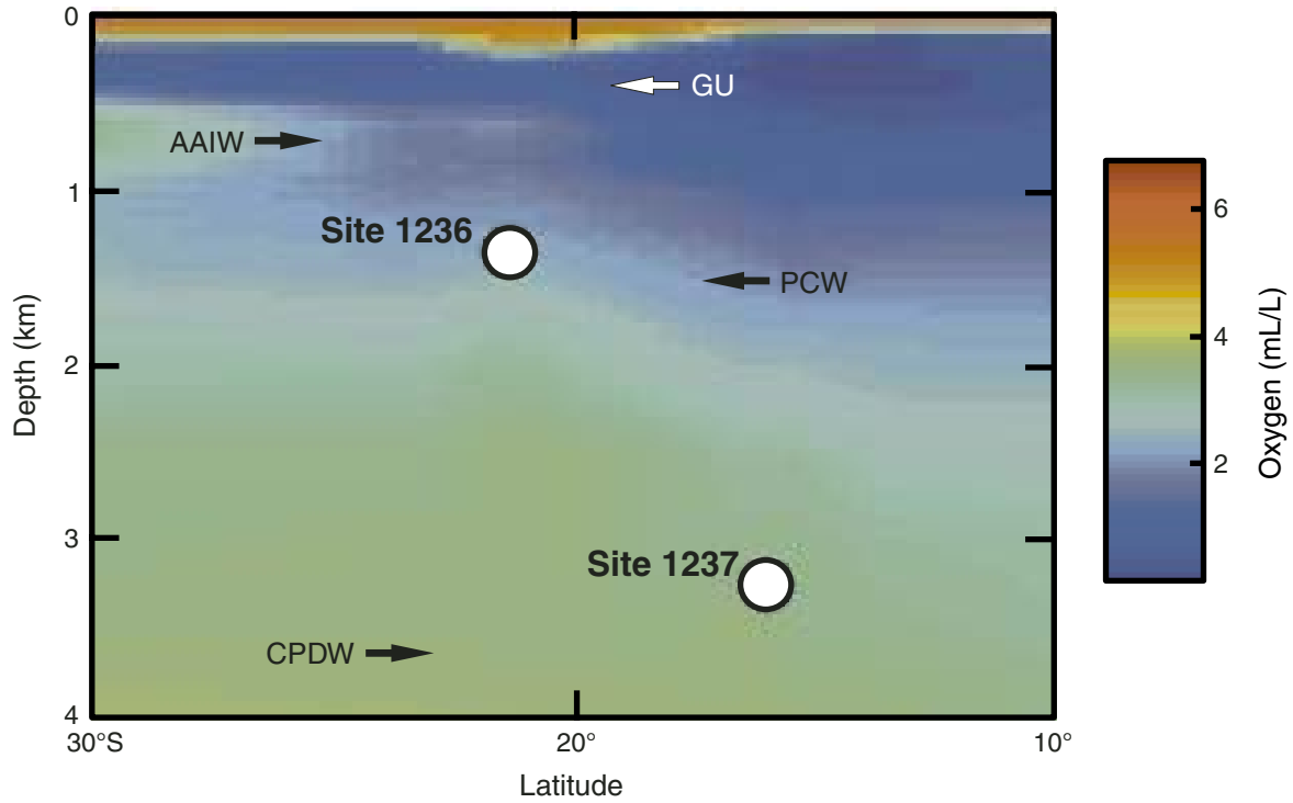
Figure F3. Meridional cross-section of southeastern Pacific (Shipboard Scientific Party, 2003) showing water masses based on dissolved oxygen concentrations (Levitus et al., 1993). Site 1237 at 3212 meters water depth is shown in relation to Pacific Central Water (PCW), Circumpolar Deep Water (CPDW), Antarctic Intermediate Water (AAIW), and Gunther Undercurrent (GU). During the late Oligocene, Site 1237 was probably at a shallower water depth and in the mixing zone between PCW and CPDW.
