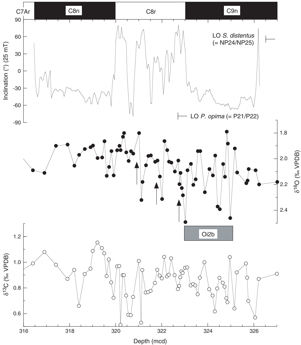
Figure F4. Magnetic polarity data (inclination after 25-mT demagnetization on the shipboard pass-through magnetometer) and stable isotope data (based on the benthic foraminifer Cibicidoides mundulus ) vs. depth in Core 202-1237B-31H. Also shown are interpreted paleomagnetic Chrons 7Ar to 9n and last occurrence (LO) of the calcareous nannofossil Sphenolithus distentus (Shipboard Scientific Party, 2003) and LO of the planktonic foraminifer Paragloborotalia opima (this study). The late Oligocene climate transition occurs as a three-step decrease in \delta^{18}\text{O} within Chron 8r (here termed the “Chron 8r \delta^{18}\text{O} shift”), immediately following Oi2b of Miller et al. (1991). VPDB = Vienna Pee Dee belemnite.
