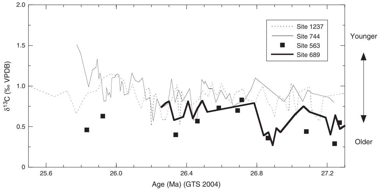
Figure F6. Stable carbon isotope data (based on Cibicides mundulus ) from southeast Pacific Site 1237 (this study), southern Indian Ocean Site 744 (Barrera and Huber, 1992), North Atlantic Site 563 (Miller and Fairbanks, 1985), and Southern Ocean Site 689 (Kennett and Stott, 1990). Higher and lower \delta^{13}\text{C} values indicate younger and older deep waters, respectively. Inter-ocean \delta^{13}\text{C} gradients are small during the late Oligocene ( <0.5\text{‰} ), but consistent with an Indo-Pacific to Atlantic aging of deep waters. VPDB = Vienna Pee Dee belemnite.
