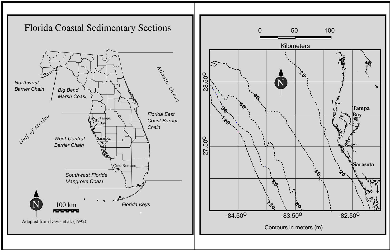
Figure 1. Florida, its coastal geomorphologic provinces (Davis et al., 1992), and bathymetry on the central West Florida Shelf.
