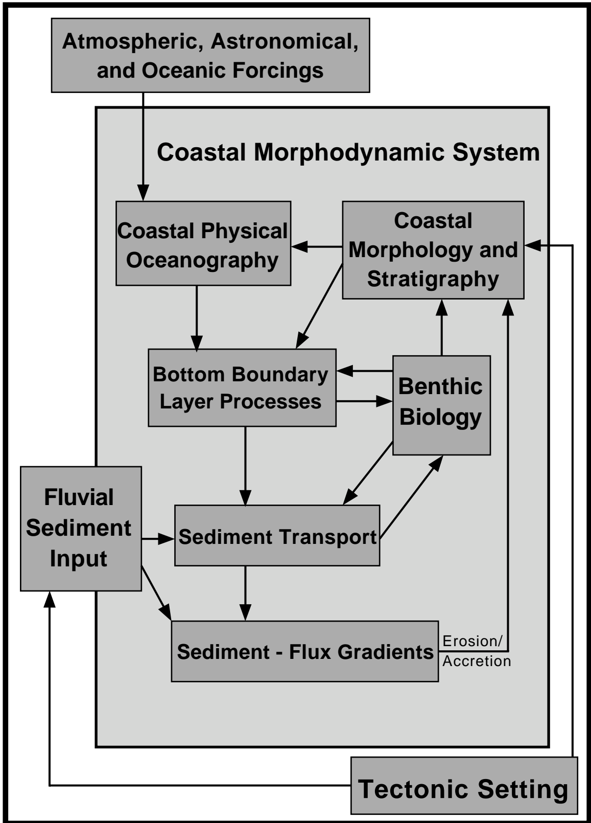
Figure 2. Flow diagram illustrating the idealized elements and linkages in a coastal morphodynamic system. (Adapted from Wright, 1995.)
