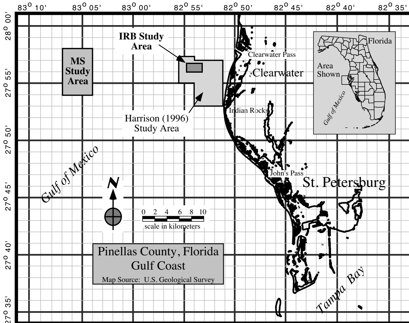
Figure 3. Location of the IRB and MS study areas in relation to the Pinellas County, FL coast. The IRB area is located within the larger study area investigated by Harrison (1996).
