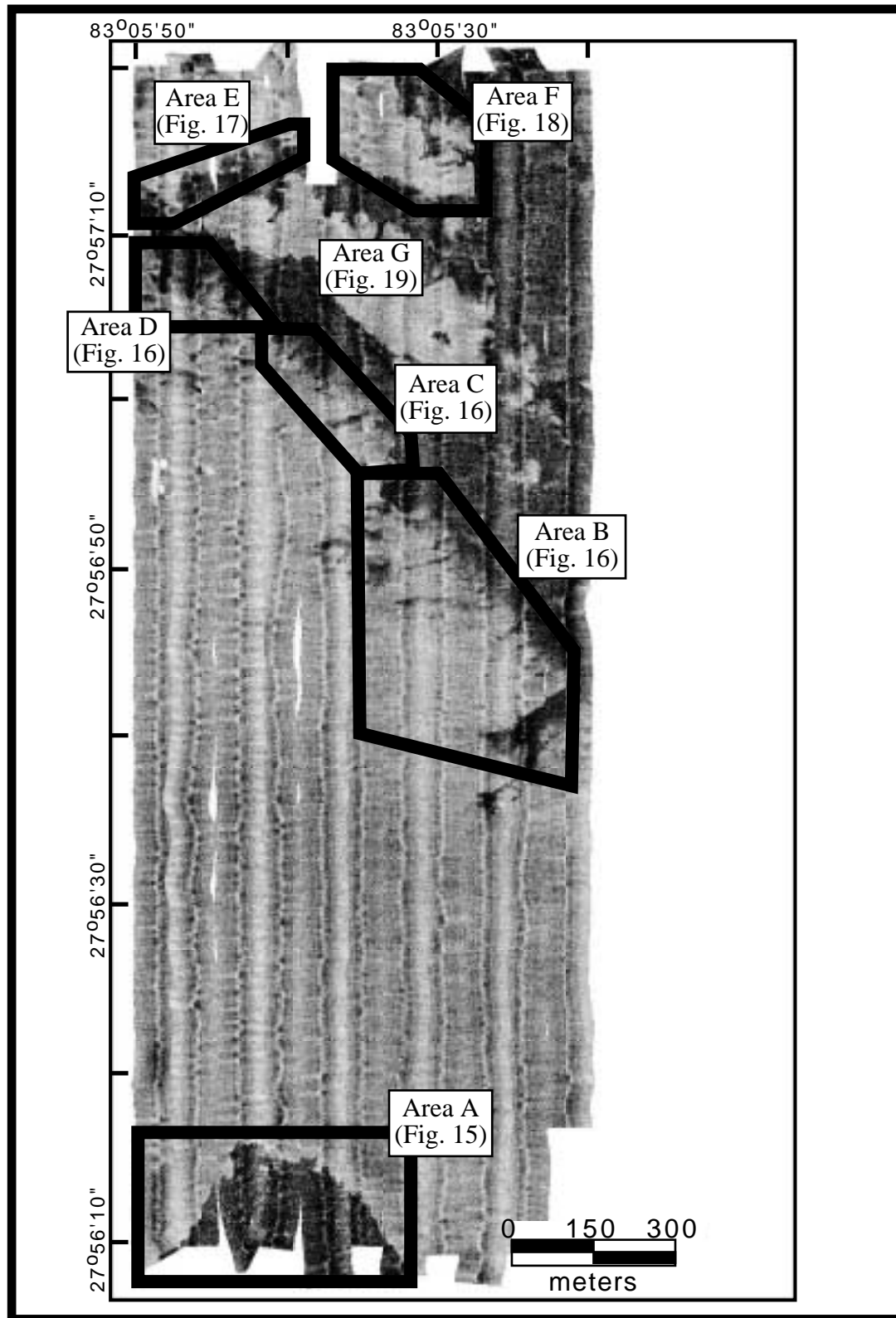
Figure 6. Locations of Midshelf (Figure 3) sub-study areas used in GIS analysis of 1996 to 1998 side-scan data.
