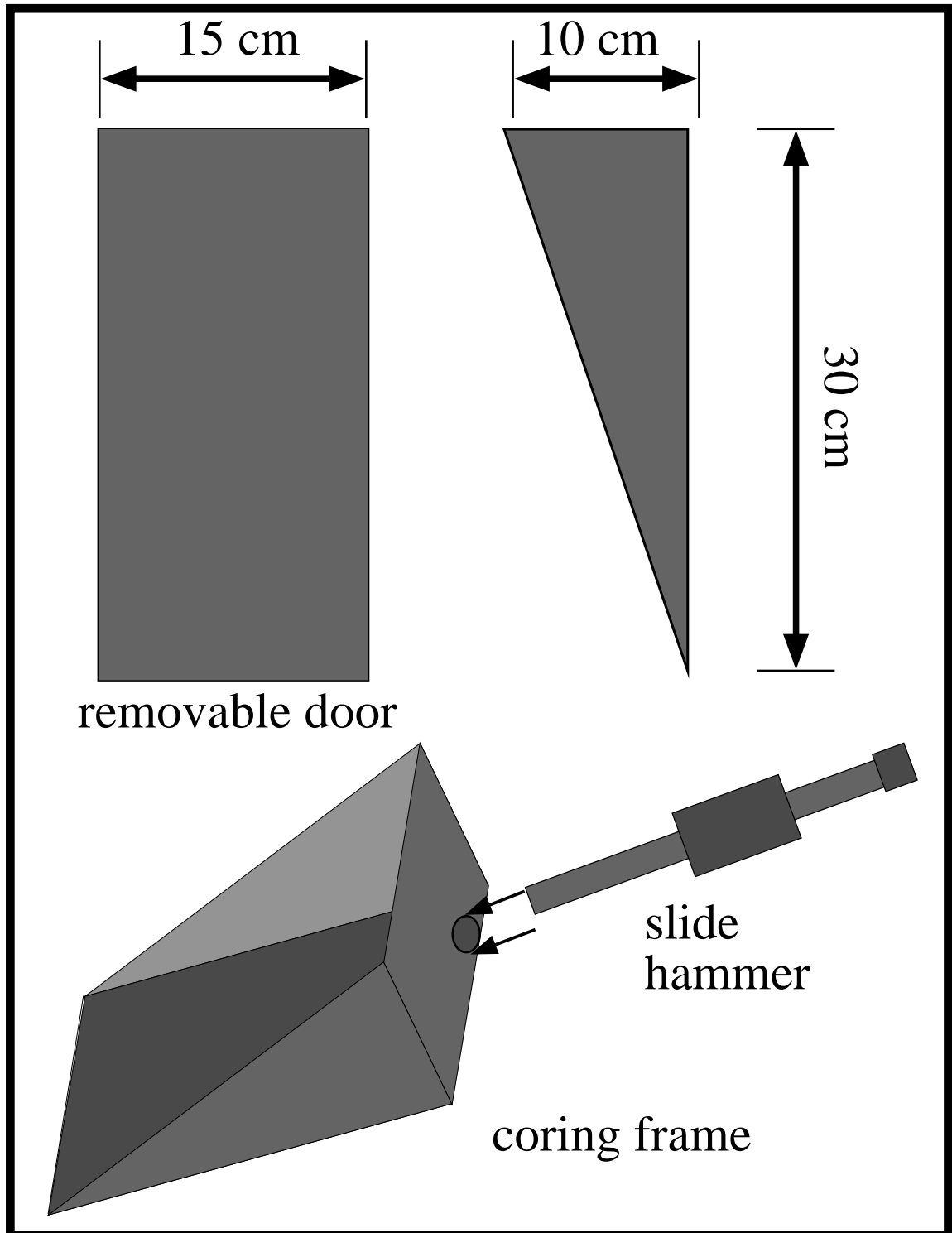
Figure 11. Diagram (not to scale) of Klován-style, diver deployed, box coring unit. The slide hammer is threaded into the coring frame. Repeated downward pounding of the hammer forces the coring frame vertically into the sediment. Once fully inserted, the core is enclosed by inserting a removable door along runners on the open side.
