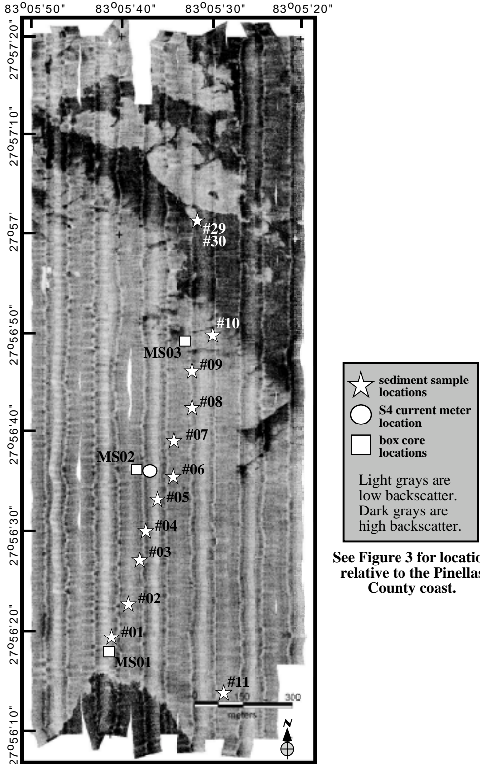
Figure 14. 500 kHz side-scan sonar mosaic from MS98JL survey.
