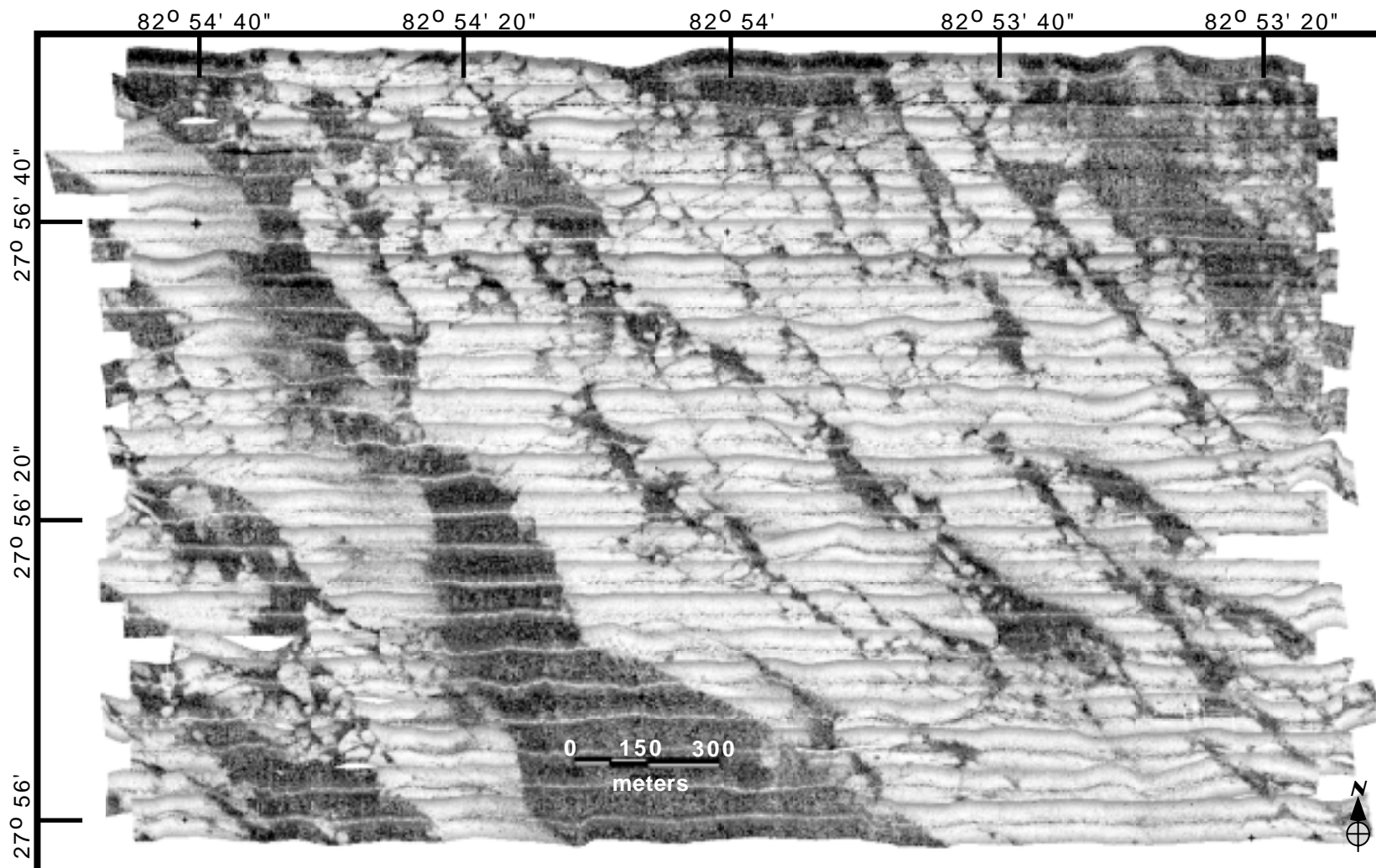
Figure 23. IRB November 1997 500 kHz side scan-sonar mosaic. See Figure 3 for location.
