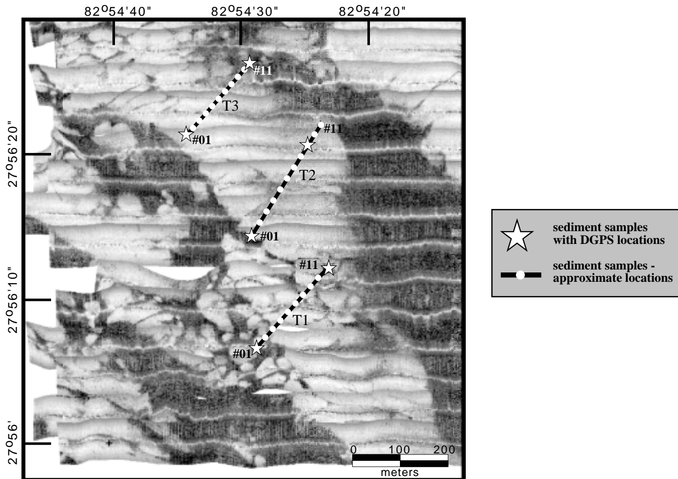
Figure 24. IRB97N sampling area (southwest sub-study area -- Figure 23). Sediment samples collected along transect T1 were ~ 24 m apart; along T2, ~30 m apart; and along T3, ~20 m apart. Note: in T1, only ten samples were collected. There was no sample #05. In T2, the DGPS fix was taken at sample #09 instead of at the end point (#11).
