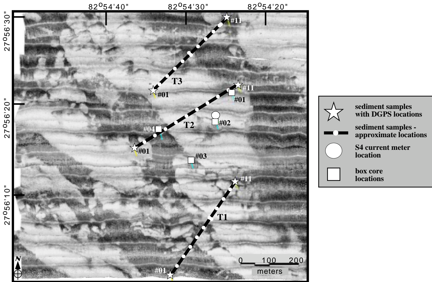
Figure 26. IRB98JL sampling area (southwest sub-study area -- Figure 25). Samples collected along transect T1 were ~24 m apart; along T2, ~30 m apart; and along T3, ~20 m apart.
