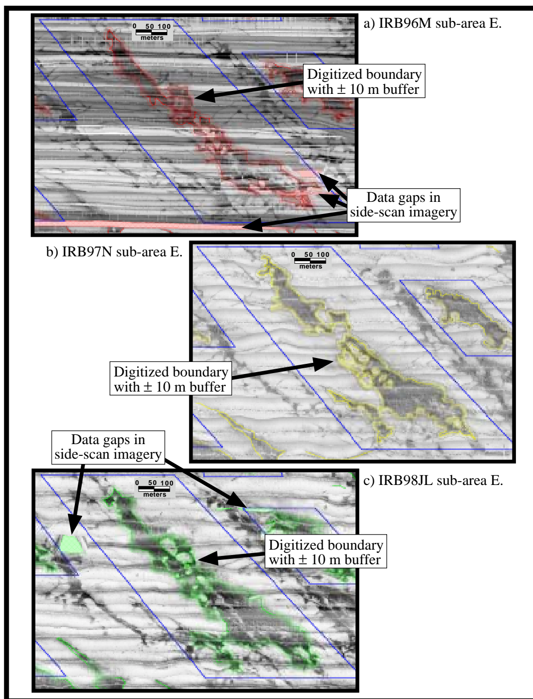
Figure 31. IRB sub-area E (Figure 7) GIS analysis. a) IRB96M side-scan image with \pm 10 m buffer along high/low backscatter boundary. b) IRB97N side-scan image with \pm 10 m buffer along high/low backscatter boundary.. c) IRB98JL side-scan image with \pm 10 m buffer along high/low backscatter boundary. (Continued on next page)
