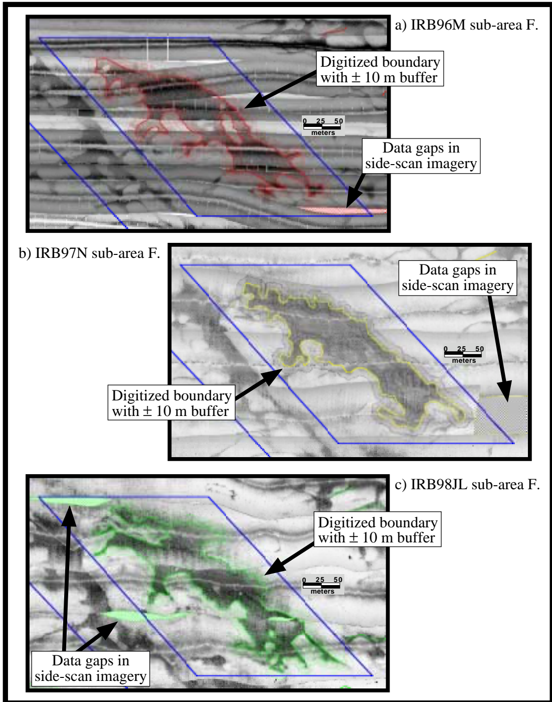
Figure 32. IRB sub-area F (Figure 7) GIS analysis. a) IRB96M side-scan image with \pm 10 m buffer along high/low backscatter boundary. b) IRB97N side-scan image with \pm 10 m buffer along high/low backscatter boundary.. c) IRB98JL side-scan image with \pm 10 m buffer along high/low backscatter boundary. (Continued on next page)
