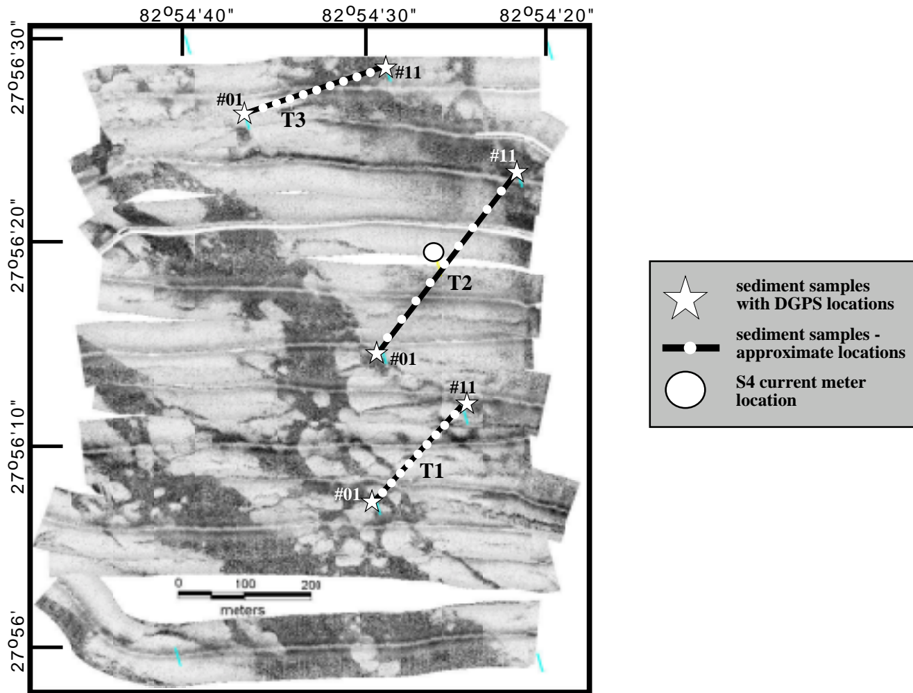
Figure 35. IRB98N2 sub-study area. Sediment samples collected along transect T1 were ~24 m apart; along T2, ~30 m apart; and along T3, ~20 m apart.
