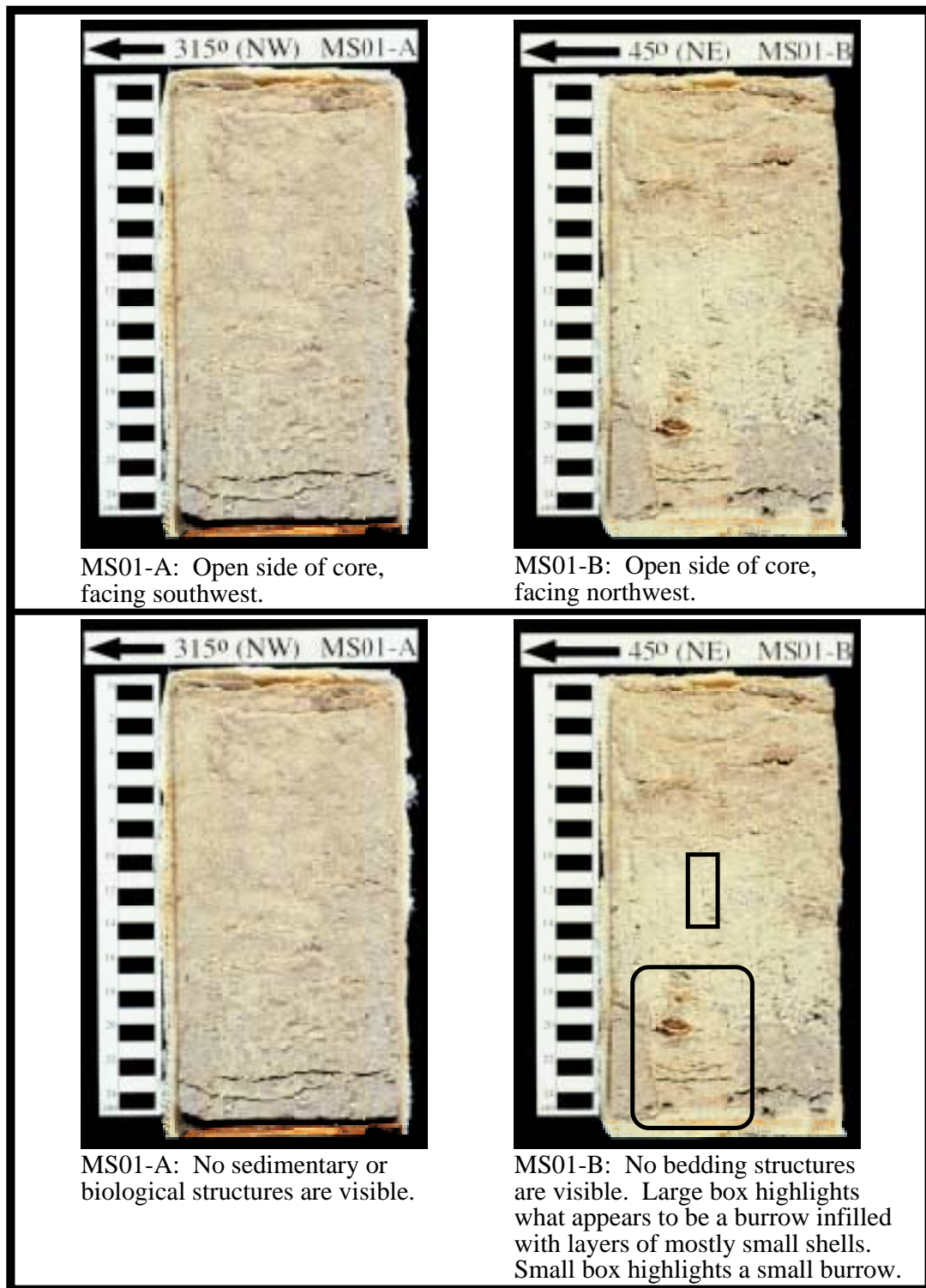
Figure 40. Embedded box core peels from site MS01 (see Figure 14 for location). Top: scans of core peels. Bottom: identification of features in each peel.
