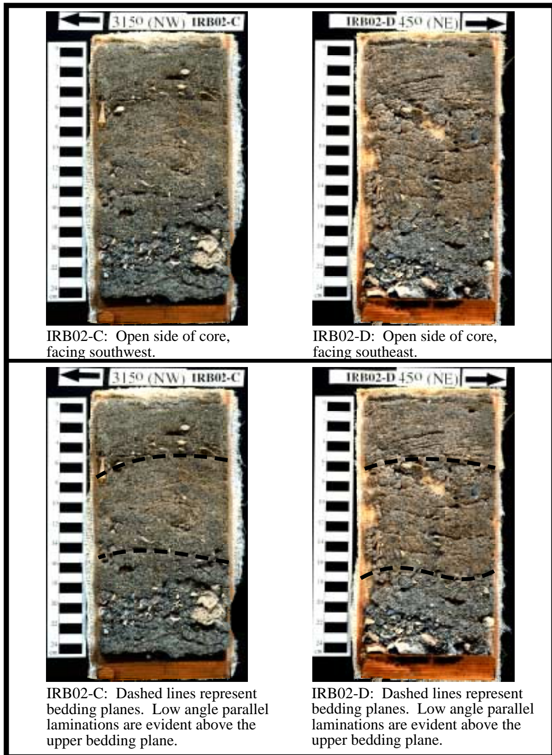
Figure 45. Embedded box core peels (November 1998) from site IRB02 (see Figure 34 for location). Top: scans of core peels. Bottom: identification of features in each core.
