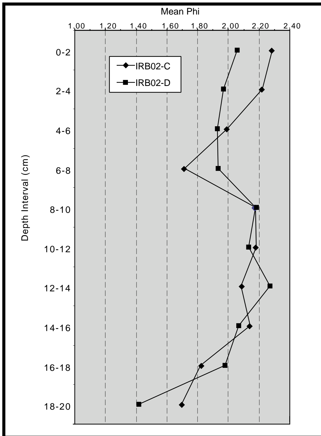
Figure 46. Mean grain size versus depth in cores IRB02-C and IRB02-D, taken in November 1998. Note the sudden coarsening of grain size at 6-8 cm depth, which corresponds with a layer of shells and coarse materials in both cores (Figure 45).
