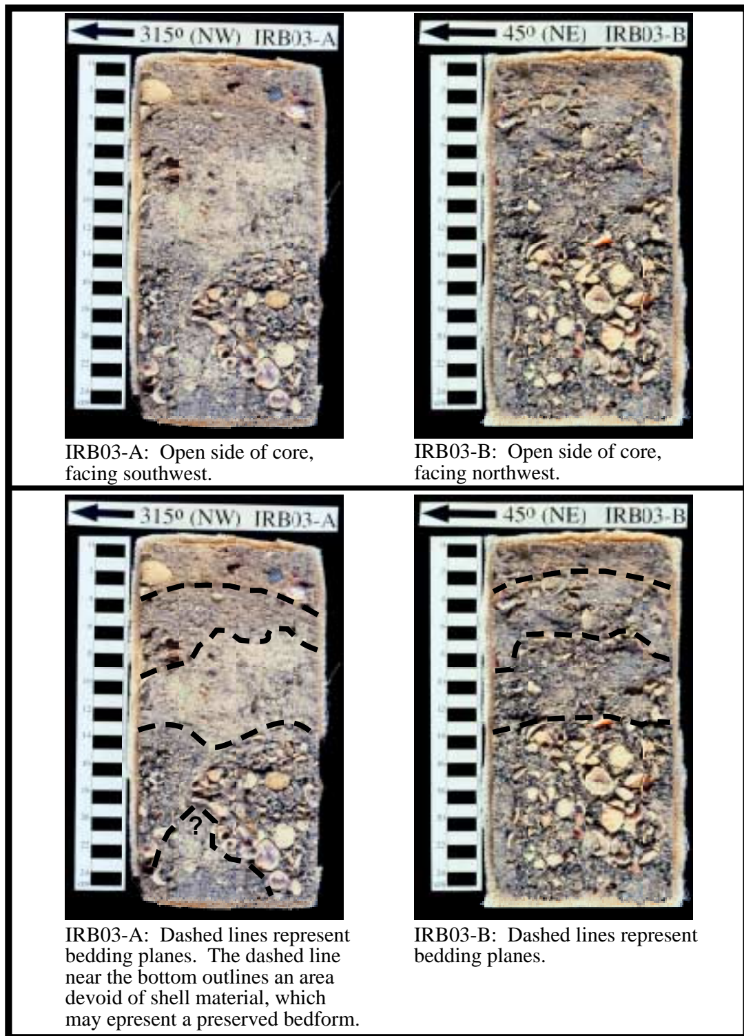
Figure 47. Embedded box core peels from site IRB03 (see Figure 26 for location). Top: scans of core peels. Bottom: identification of features in each core.
