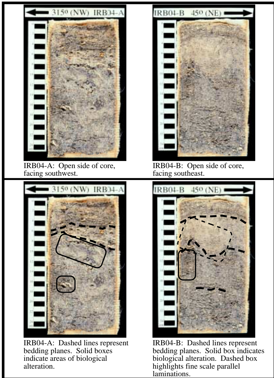
Figure 48. Embedded box core peels from site IRB04 (see Figure 26 for location). Top: scans of core peels. Bottom: identification of features in each core.
