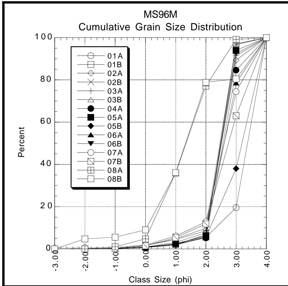
Figure 49. Cumulative frequency grain size distribution, MS96M sediment samples.
