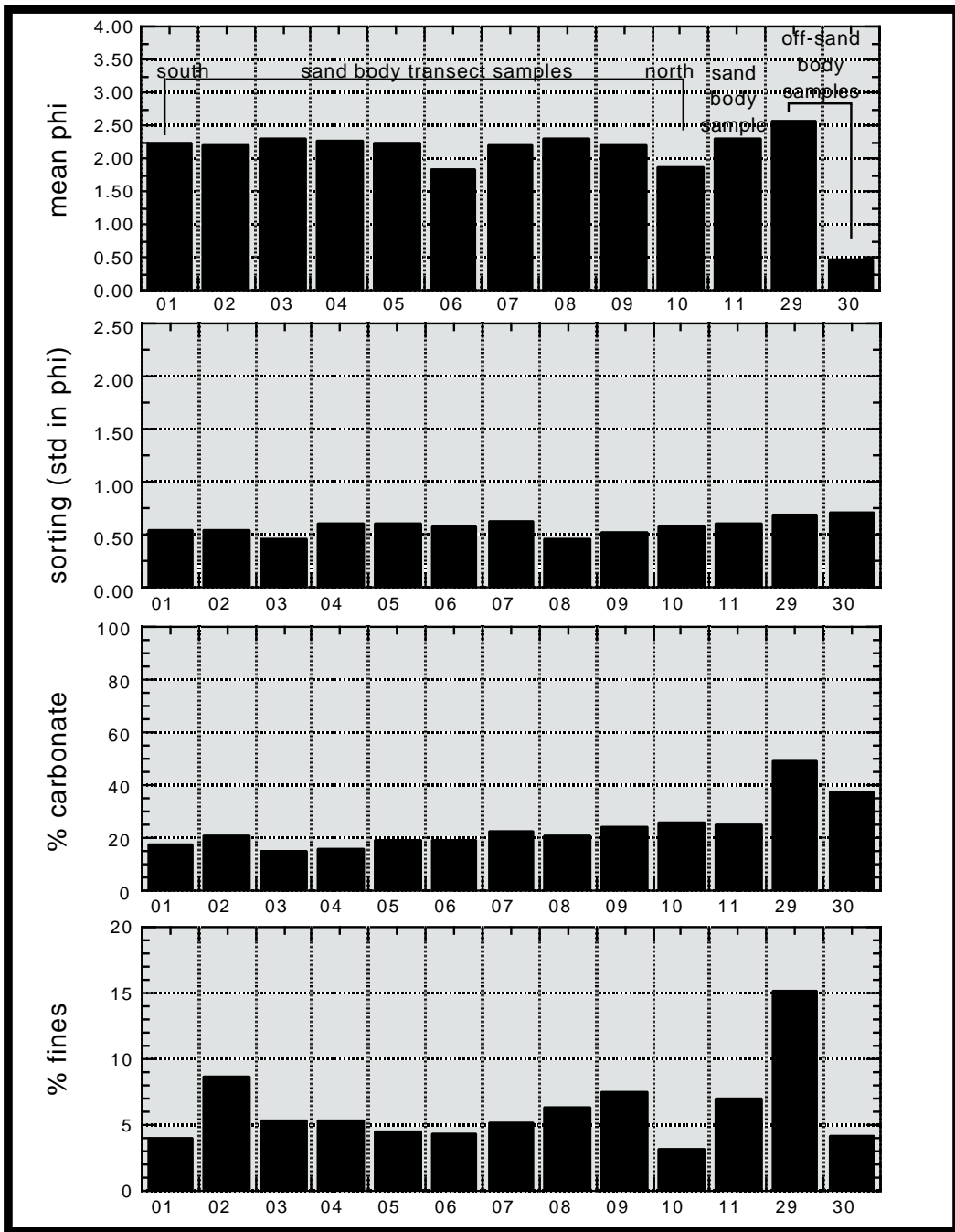
Figure 52. Comparison of sedimentary properties, MS98JL. Samples 01-10 were taken from south to north across the sand body in the MS area (Figure 14). Sample 11 was taken on the southern edge of the sand body. Samples 29 and 30 were taken north of the sand body in an area of transition. There is little variation in the sedimentary properties of the samples from the sand body, except in the percentage of the fine fraction. The trough samples show higher percent carbonate, and vary in mean \phi and fines, but not in sorting.
