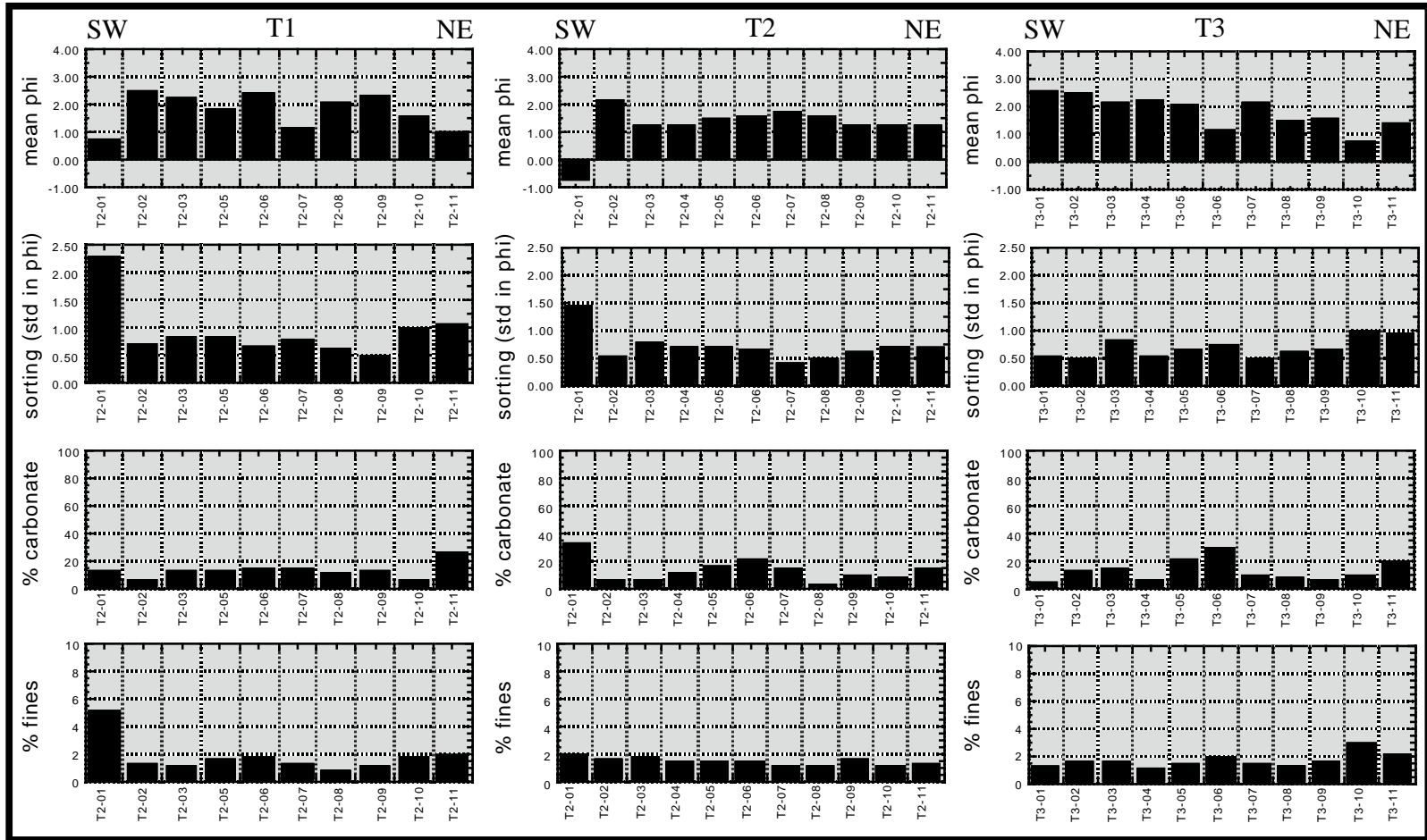
Figure 54. Comparison of sedimentary properties for IRB97N samples, taken from SW (-01) to NE (-11) along three transects (T1, T2, and T3) (Figure 24). Sorting is the standard deviation in phi units (Folk, 1980). Percent carbonate is by weight of the sand size fraction only. Percent fines is by weight of the the entire sample. There is some correlation between carbonate content and sorting, with samples being more poorly sorted the more carbonate they contain. There is little variation in the amount of fine material in each sample. Note: there is no sample labeled T1-04.
