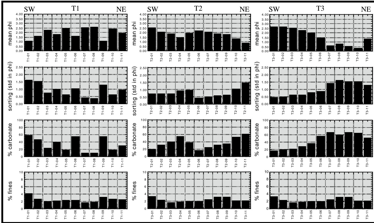
Figure 60. Comparison of sedimentary properties for IRB98N2 samples, taken from SW (-01) to NE (-11) along three transects (T1, T2, and T3) (Figure 35). Sorting is the standard deviation in phi units (Folk, 1980). Percent carbonate is by weight of the sand size fraction only. Percent fines is by weight of the entire sample. Higher carbonate content appears to correlate with poorer sorting in samples from all three transects; there also appears to be a stronger relationship between sorting and mean grain size than observed in other sample sets.
