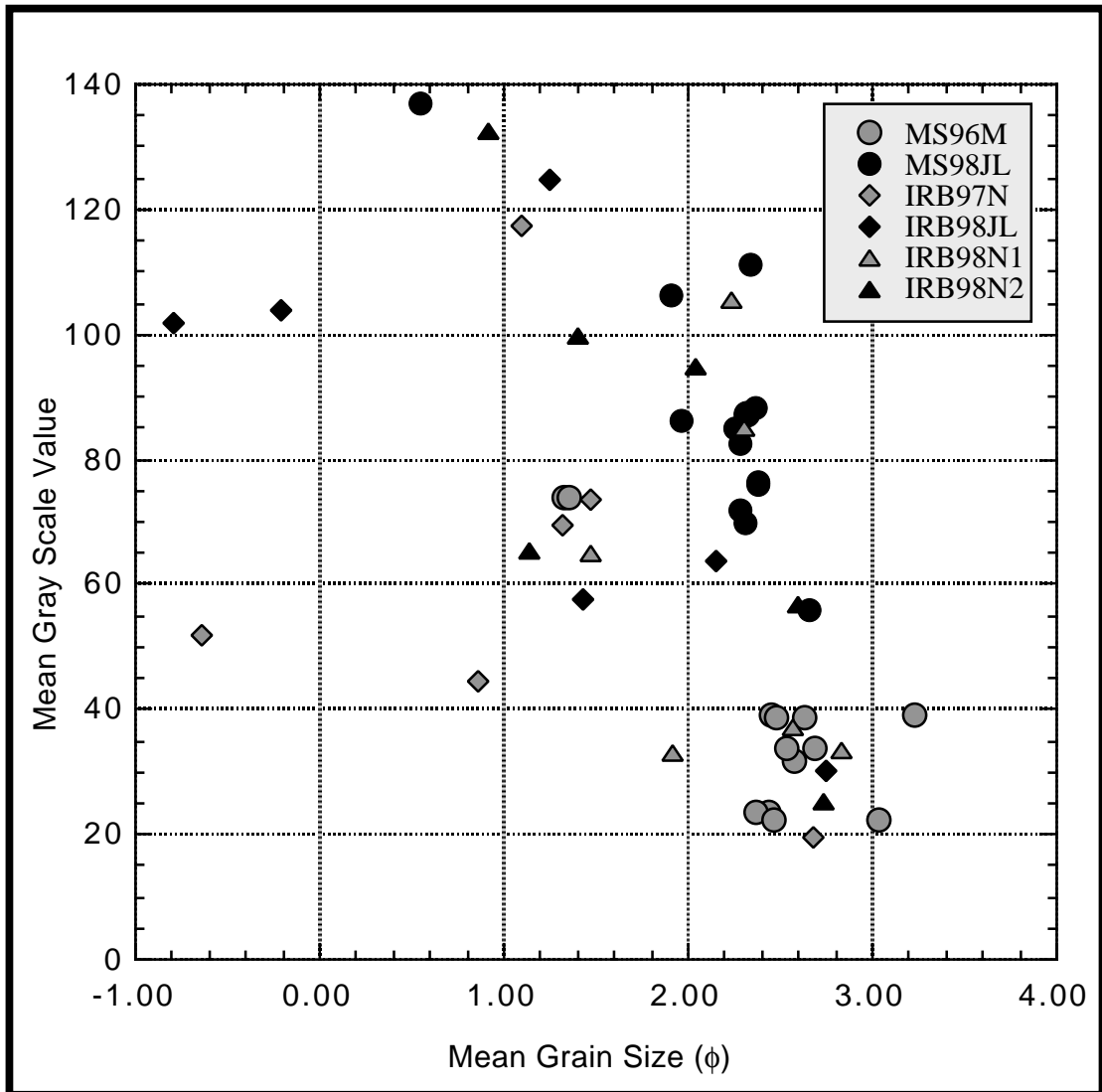
Figure 62. Mean grain size plotted against mean gray scale value for sediment samples with DGPS locations from all data sets.
