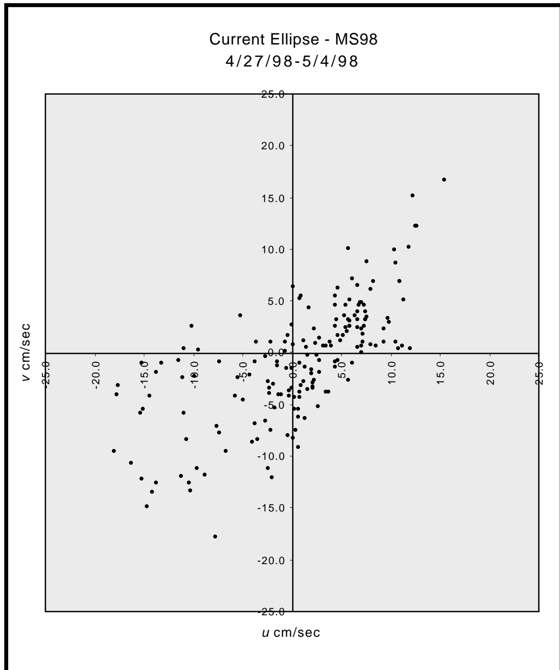
Figure 69. Current ellipse for MS98S4 data. East-west ( u ) component plotted against the north-south ( v ) component exhibited a northeasterly-southwesterly trend in the mean current vectors, which is approximately perpendicular to the axes of the sand bodies in the MS area (Figure 14).
