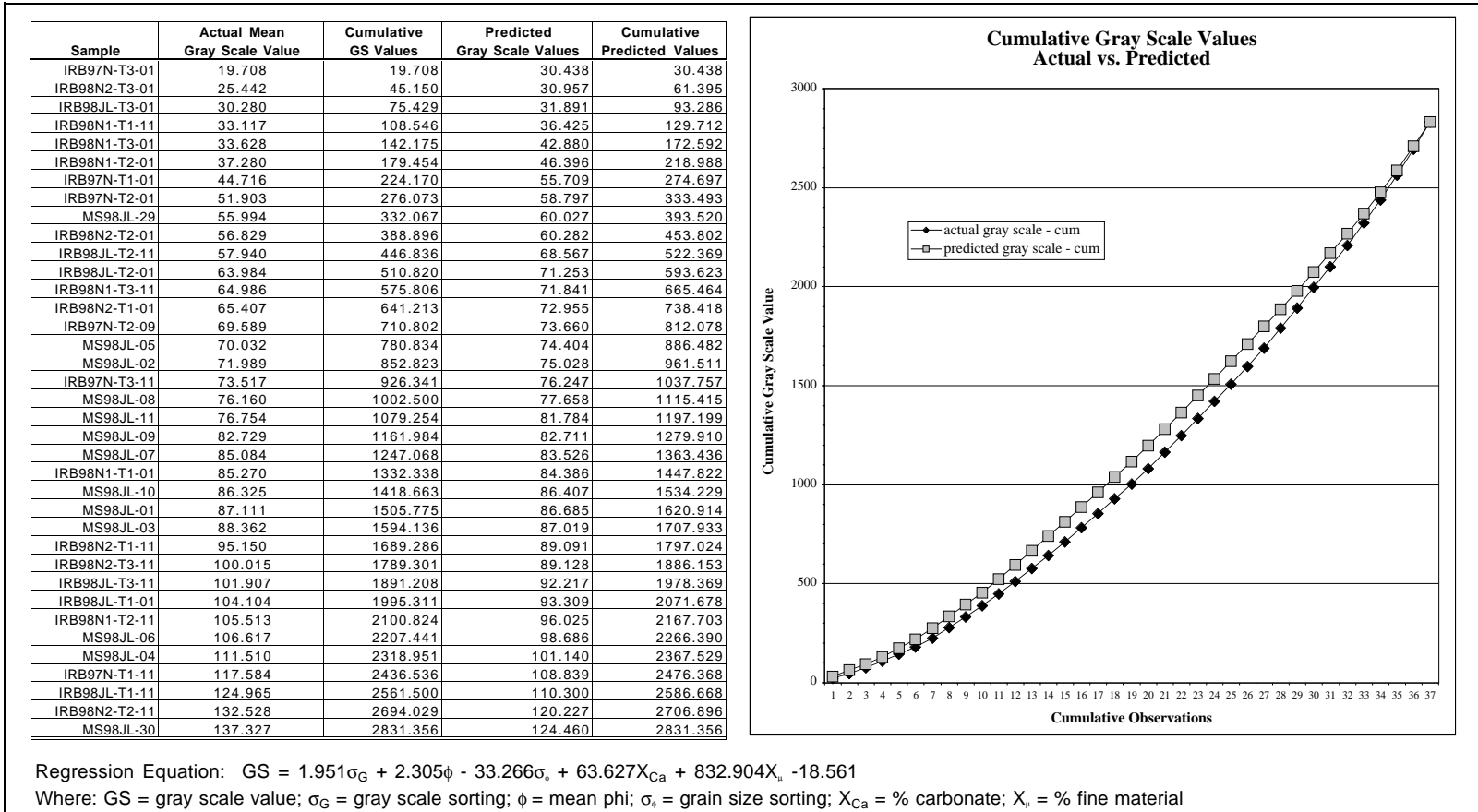
Figure 79. Actual and predicted mean gray scale values for all 500 kHz side-scan/sediment sampling sites. The cumulative table and graph of cumulative values suggests that the regression equation overpredicts gray scale for values in the lower ranges (under ~85),
