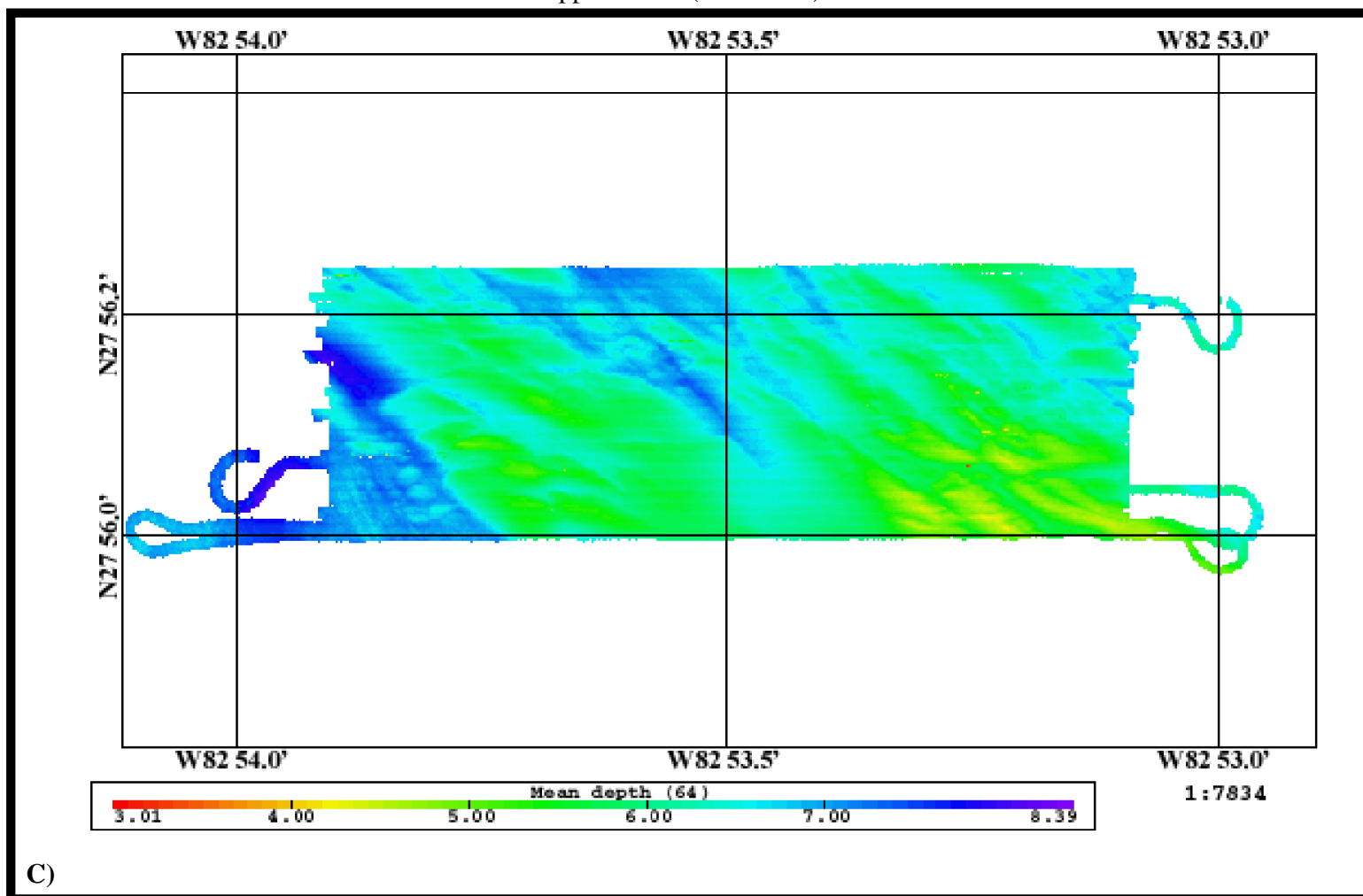
C) Partial swath bathymetry from IRB study area (Figure 3), collected in March 1999.
