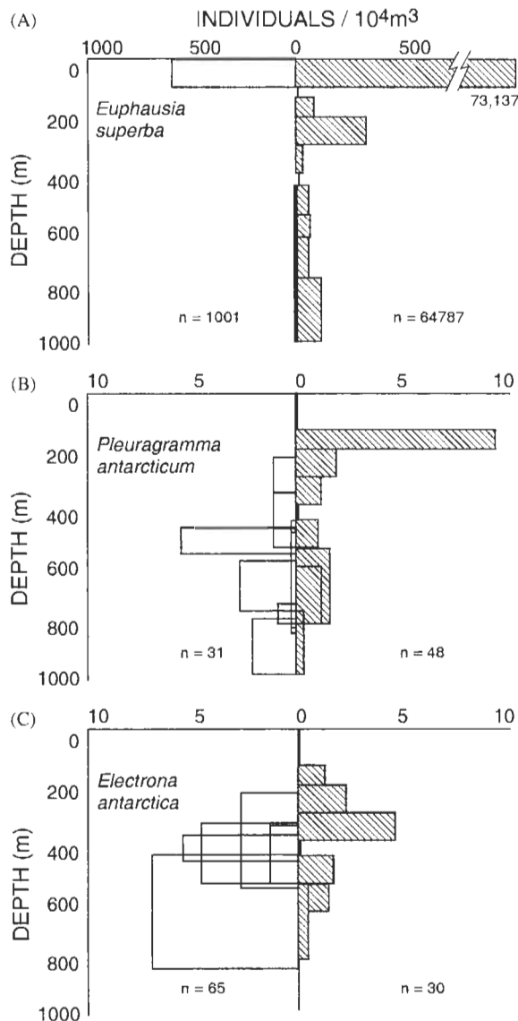
Fig. 2. Diel depth abundance patterns (individuals/10 4 m 3 ) of Euphausia superba (A) and its major fish predators P. antarcticum (B) and Electrona antarctica (C) in the Croker Passage. Shaded bars are night abundances, n = total number of individuals in day or night samples.
